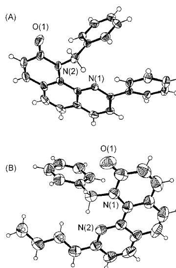
Figure 1. (A) ORTEP view with partial numbering of compound 5b , thermal ellipsoids include 50% of the electron density. (B) ORTEP view with partial numbering of compound 5d , thermal ellipsoids include 30% of the electron density.
