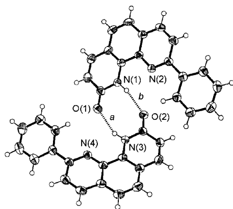
Figure 2. ORTEP view with partial numbering of the H-bonded dimer of compound 7d , thermal ellipsoids include 50% of the electron density ( a : 2.108 Å; b : 2.168 Å).
